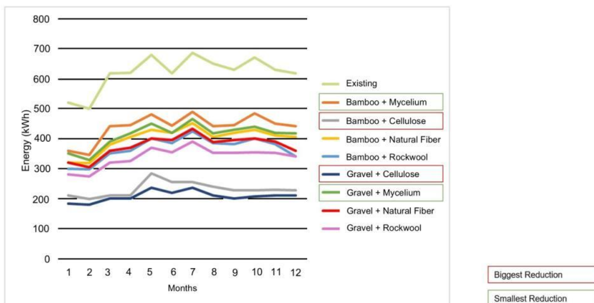
Figure 7. Comparative simulation of cooling energy load consumption
