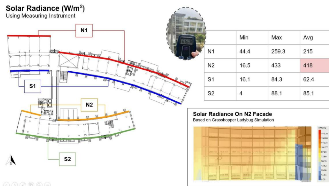
Figure 4. Solar measurement
