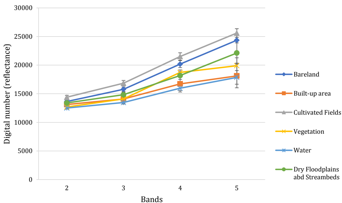
Figure 6. Spectral response plot of 2017 land cover types
